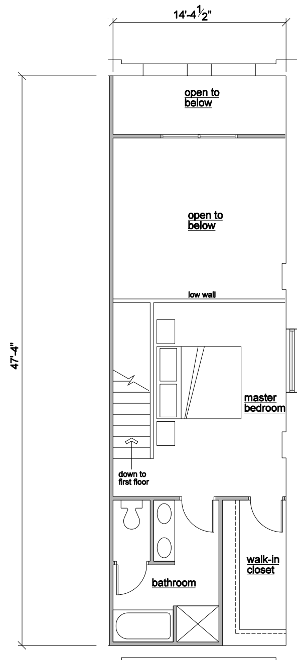
Second Floor 469 s.f.
