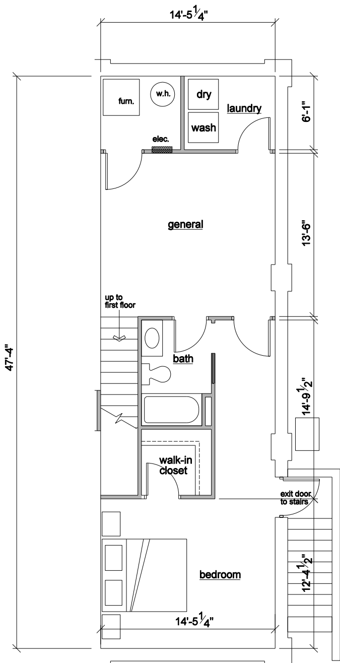
Lower Level 777 s.f.
