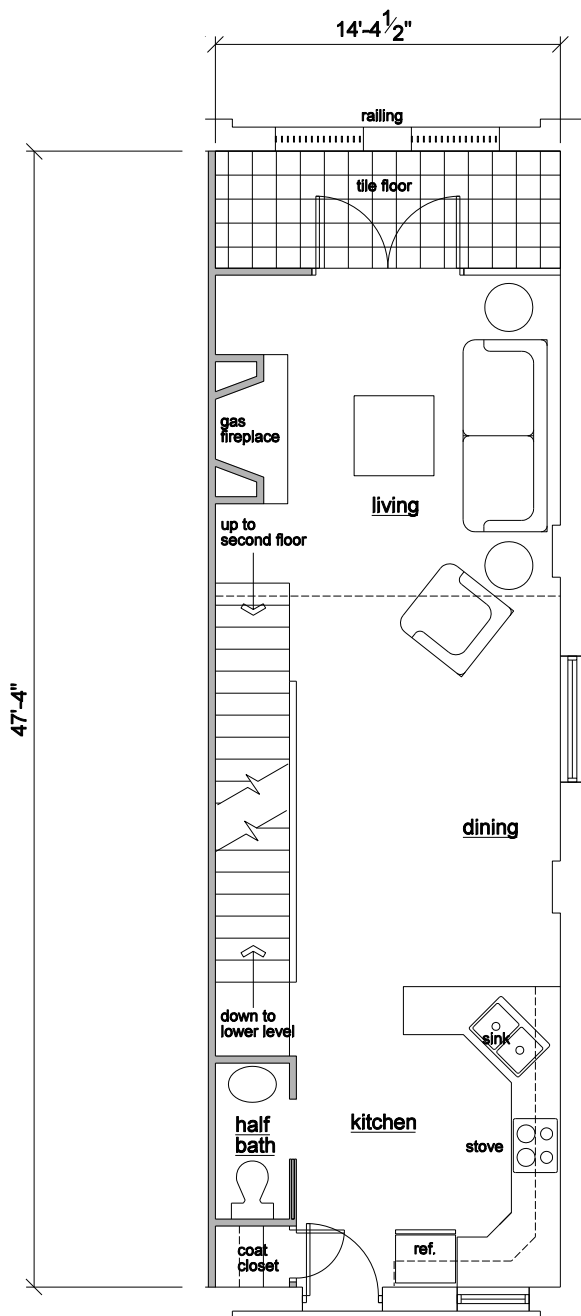
First Floor 777 s.f.
