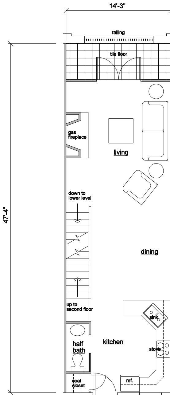
First Floor 740 s.f.
