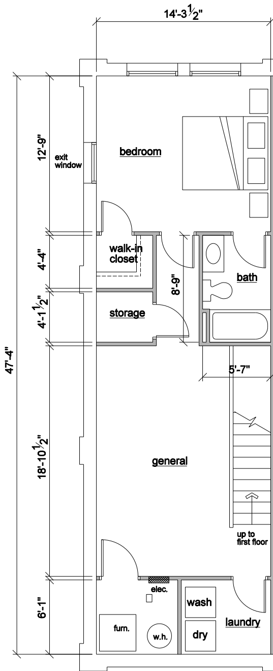
Lower Level 773 s.f.
