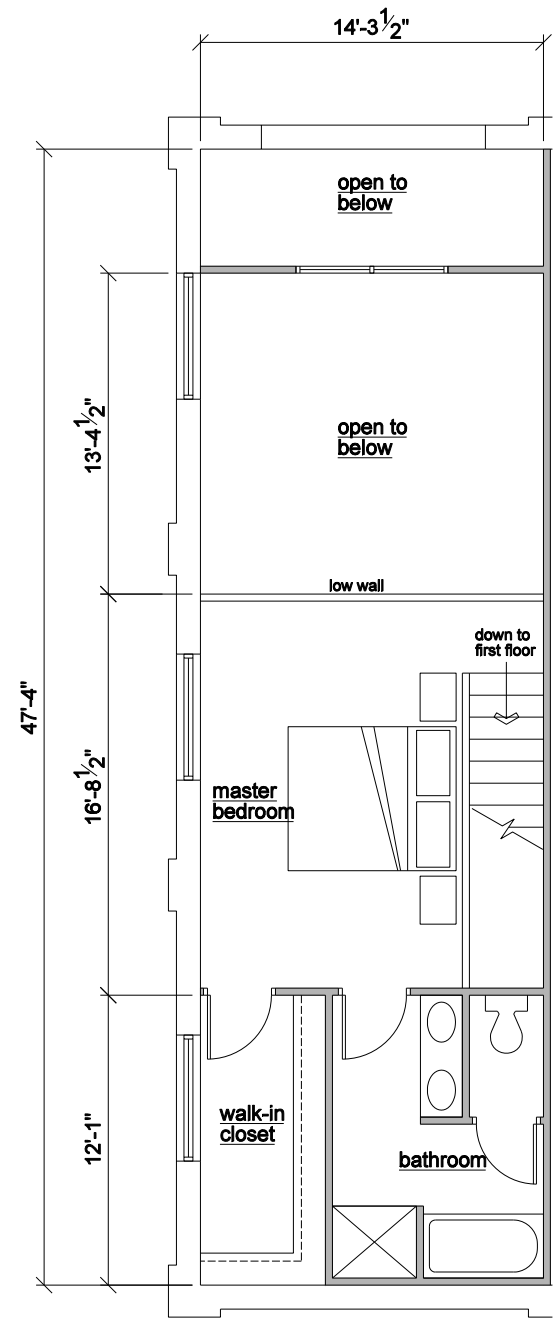
Second Floor 467 s.f.
