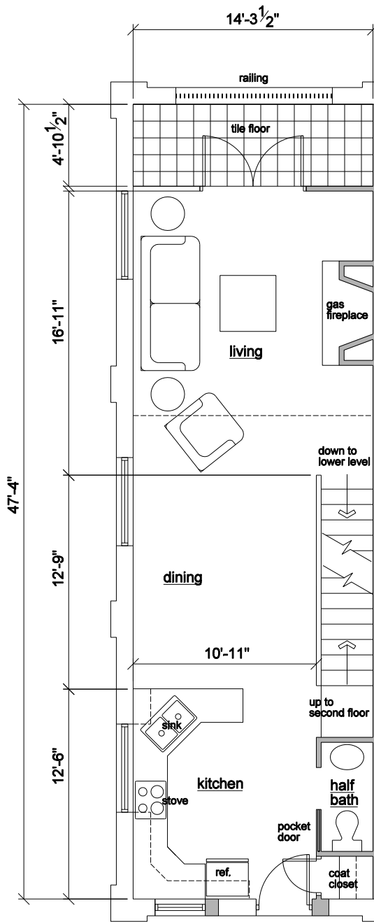
First Floor 773 s.f.
